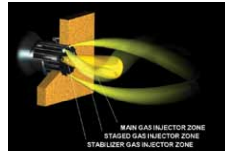
Advanced CFD modeling on every burner
