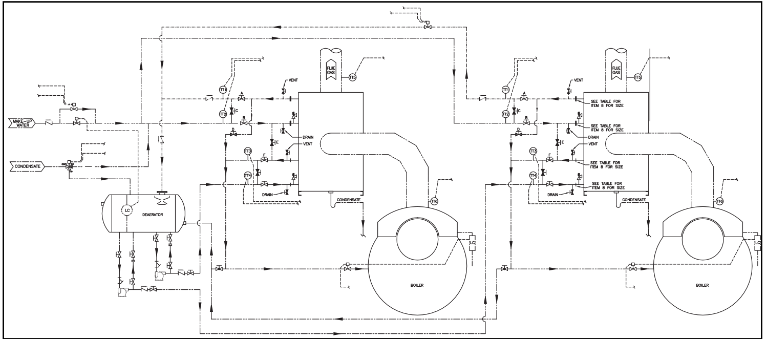
Figure 5 - Typical system piping: two boilers and deaerator
