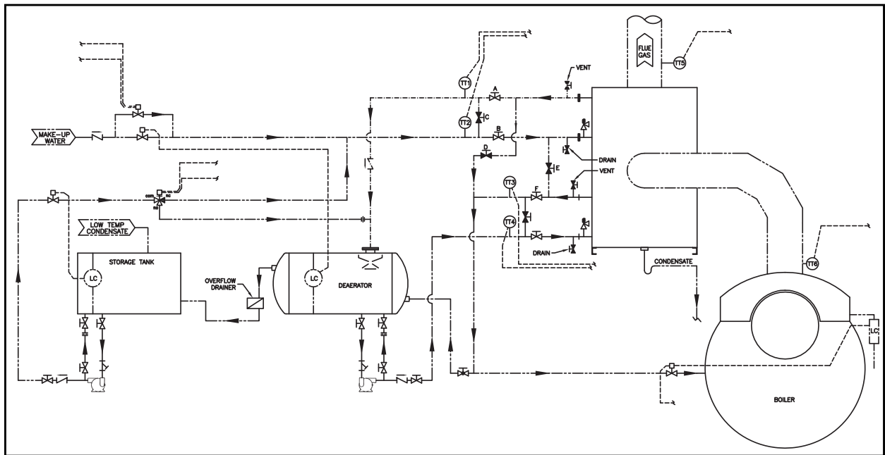
Figure 4 - Typical system piping: single boiler, deaerator, and surge tank
