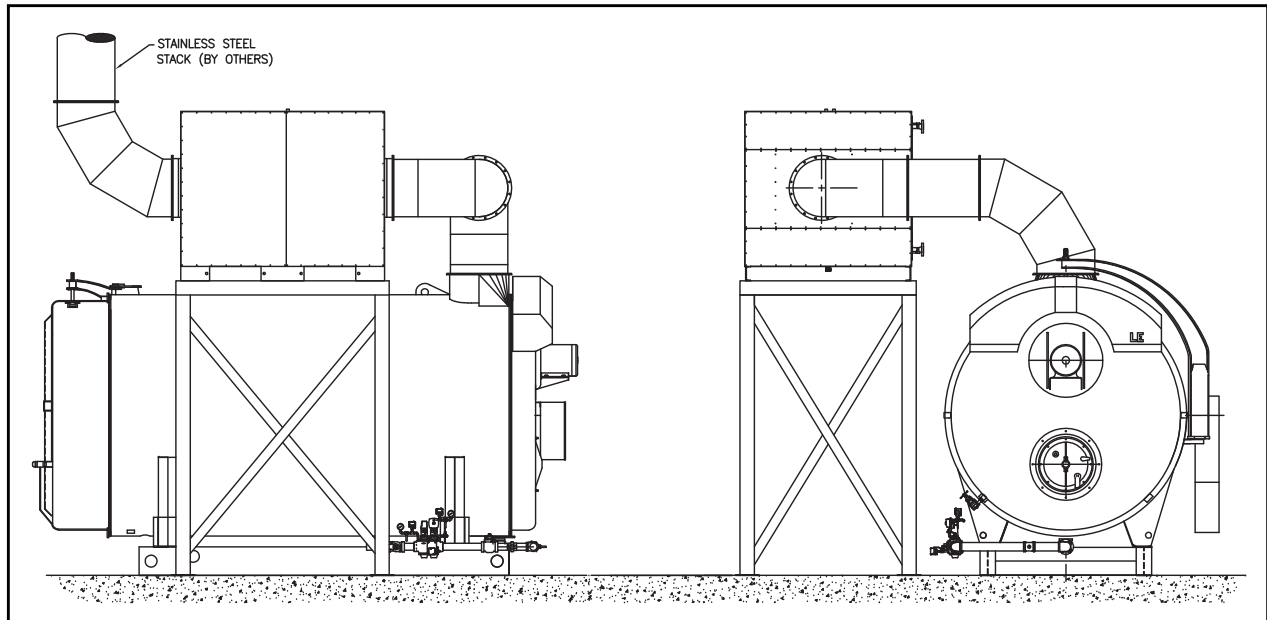
Figure 2 - Installation, typical
