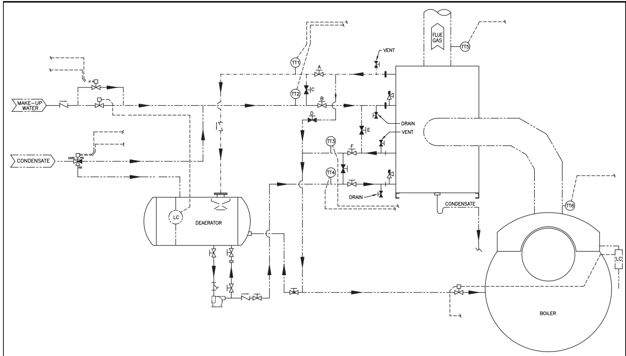
Figure 3 - Typical system piping: single boiler and deaerator
