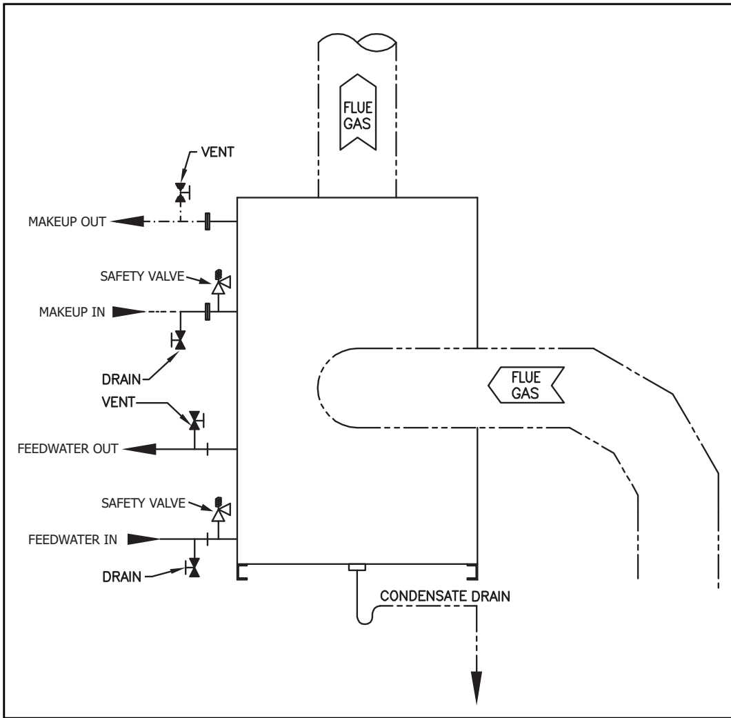
Figure 7 - Economizer piping detail
