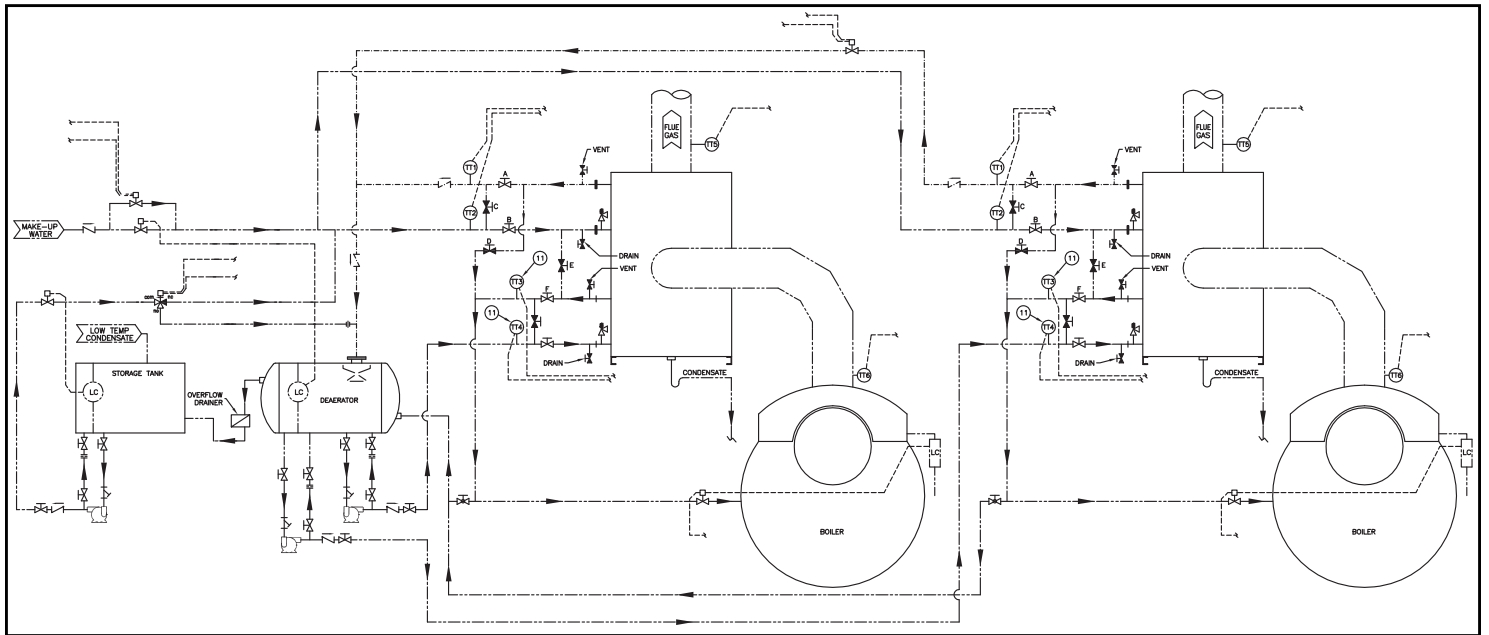
Figure 6 - Typical system piping: two boilers, deaerator, and surge tank
